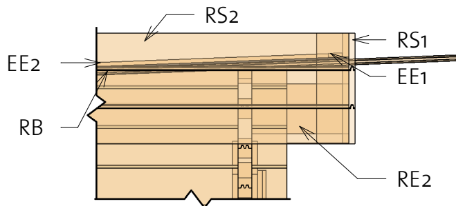
2 Roof - Callout Front
